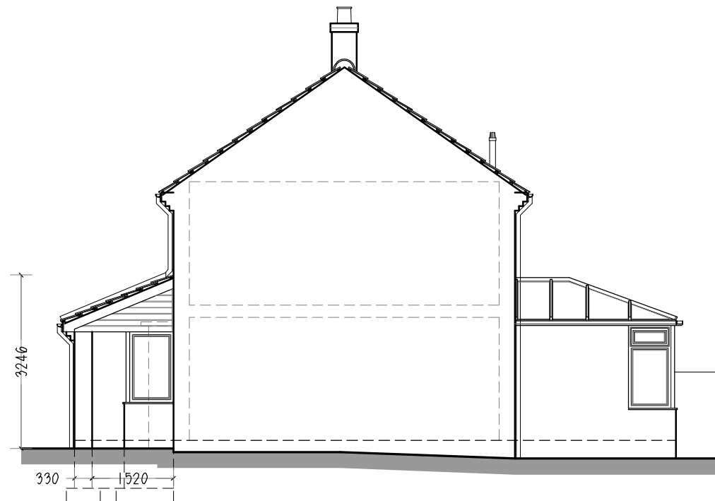
PROPOSED SIDE/ N.W. ELEVATION 1:100
